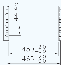
Mounting dimension
